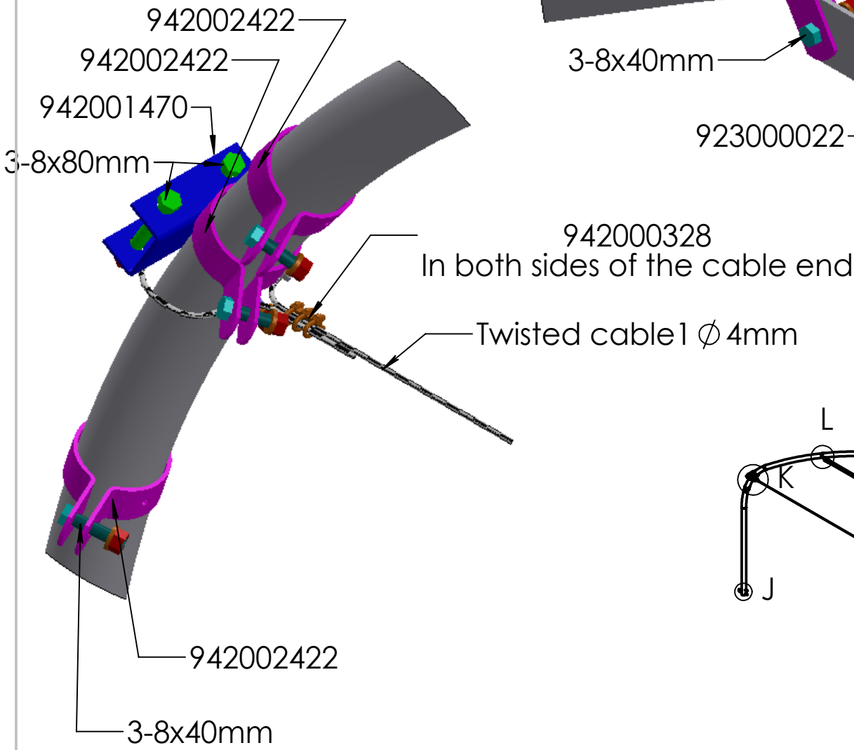
DETAIL J
