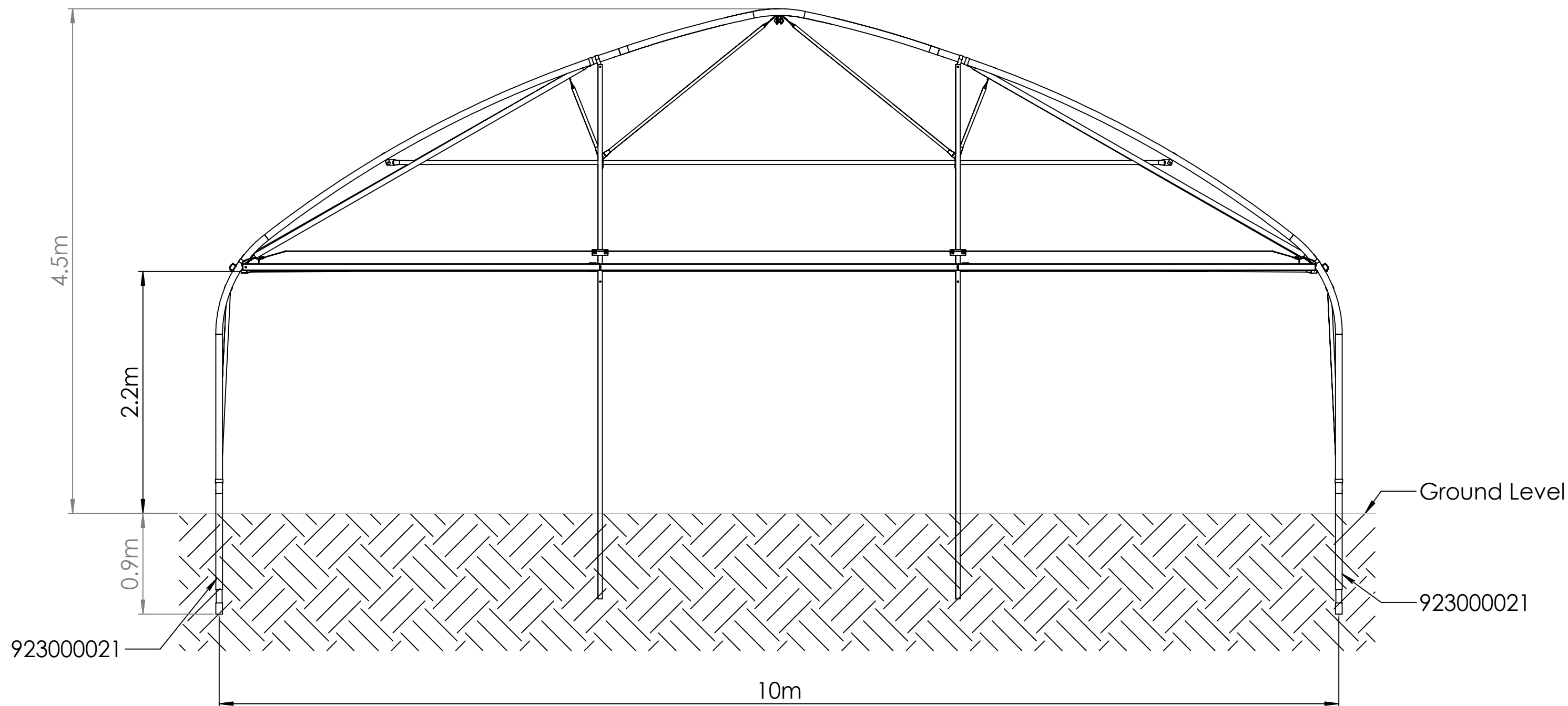
FRONT VIEW
